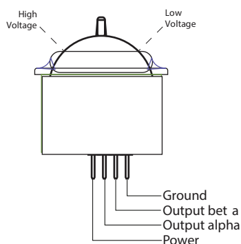
CONNECTOR PINOUT
