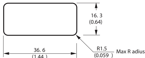
PANEL CUT-OUT
