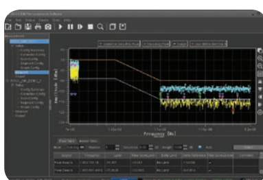
EMI预一致性测试软件 ( S1210 EMI Pre-compliance Software )
