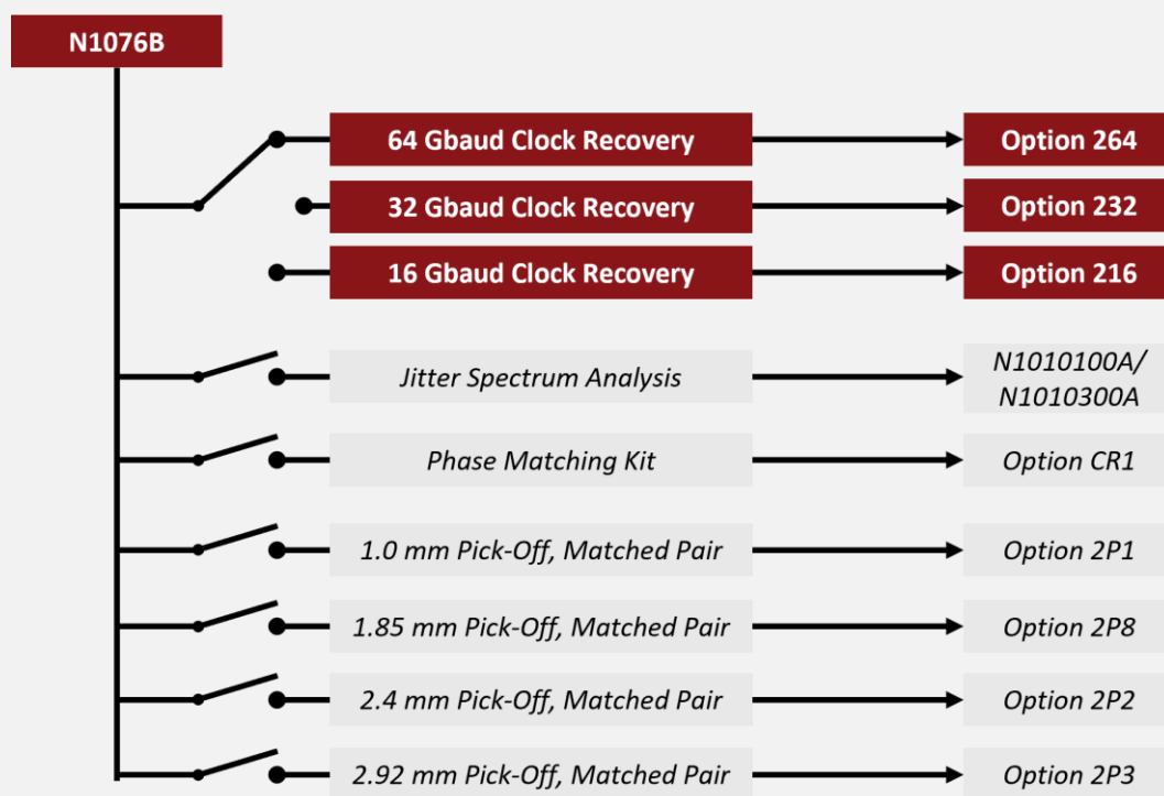
Figure 20. N1076B Electrical clock recovery with option 264
