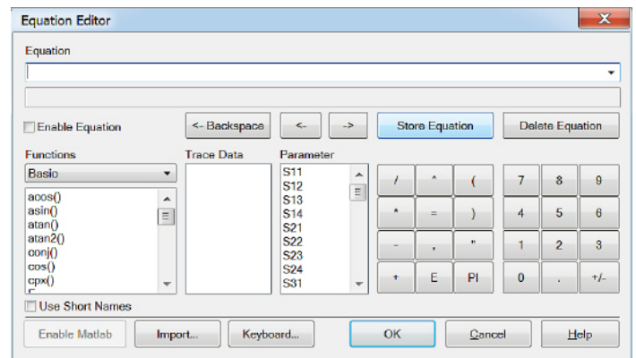
Figure 13. Equation editor
