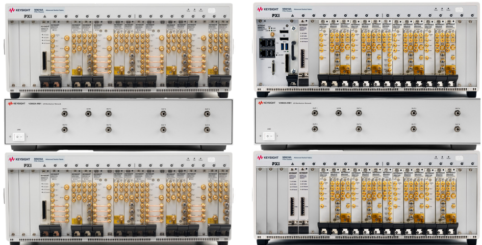
Figure 9. 8-channel PXIe VSG and 8-channel PXIe VSA with two V2802A LO distribution networks for phase coherency beyond 4 channels
