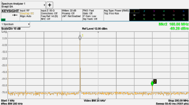
Figure 3. Single-tone spectrum @ f out = 80 MHz
