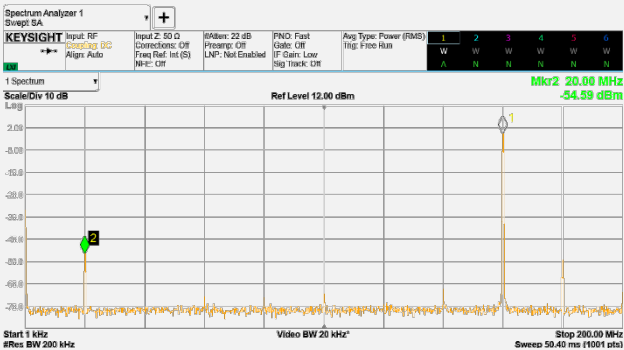
Figure 5. Single-tone spectrum @ f out = 160 MHz
