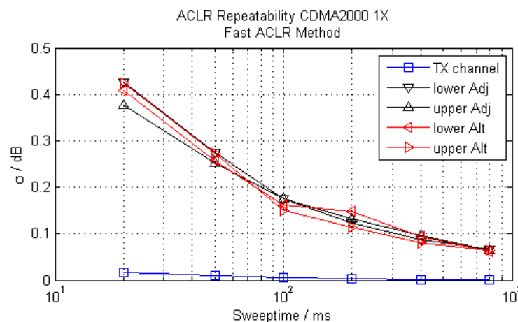
Figure 11-4: Repeatability of adjacent channel power measurements on CDMA2000 signals in the fast ACP mode
