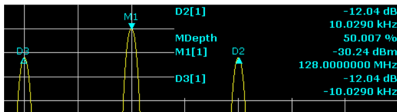
Figure 8-7: Measurement of the AM modulation depth
