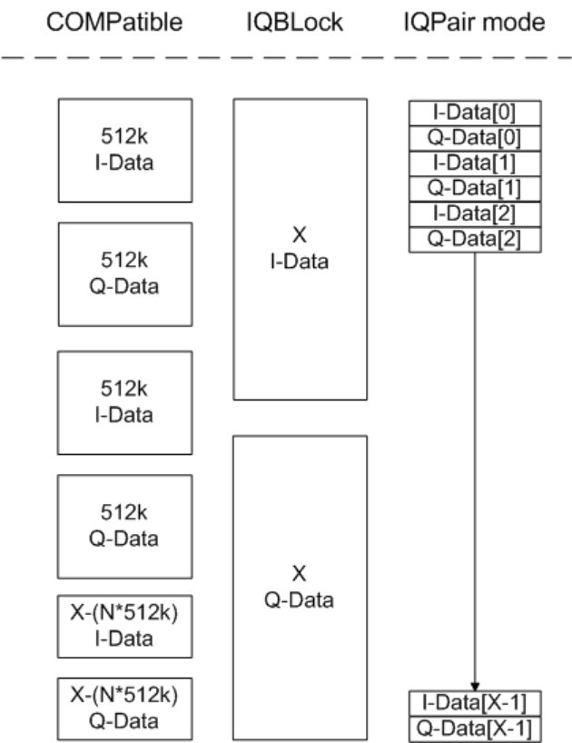
Figure 16-5: IQ data formats
