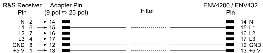
Figure 10-8: Connection from R&amp;S ESRP to R&amp;S ENV4200 or R&amp;S ENV432
