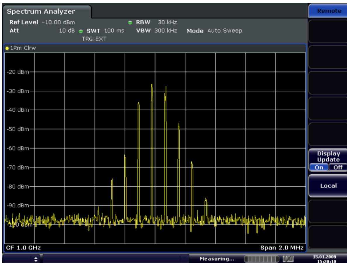
Figure 11-14: TDMA signal with GATE OFF
