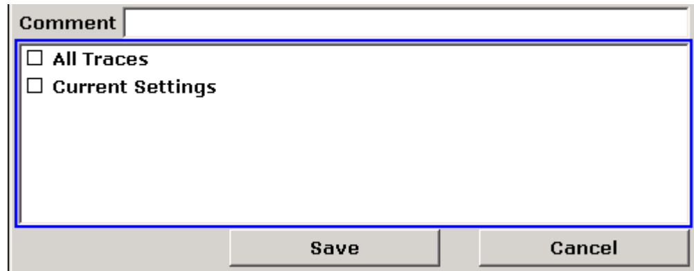
Figure 7-3: Focused area
