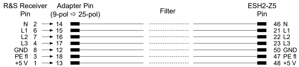
Figure 10-5: Connection from R&amp;S ESRP to R&amp;S ESH2-Z5
