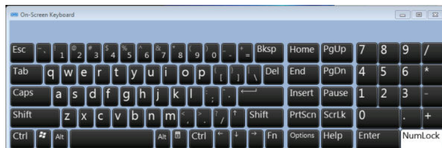
Figure 7-2: On-screen keyboard
