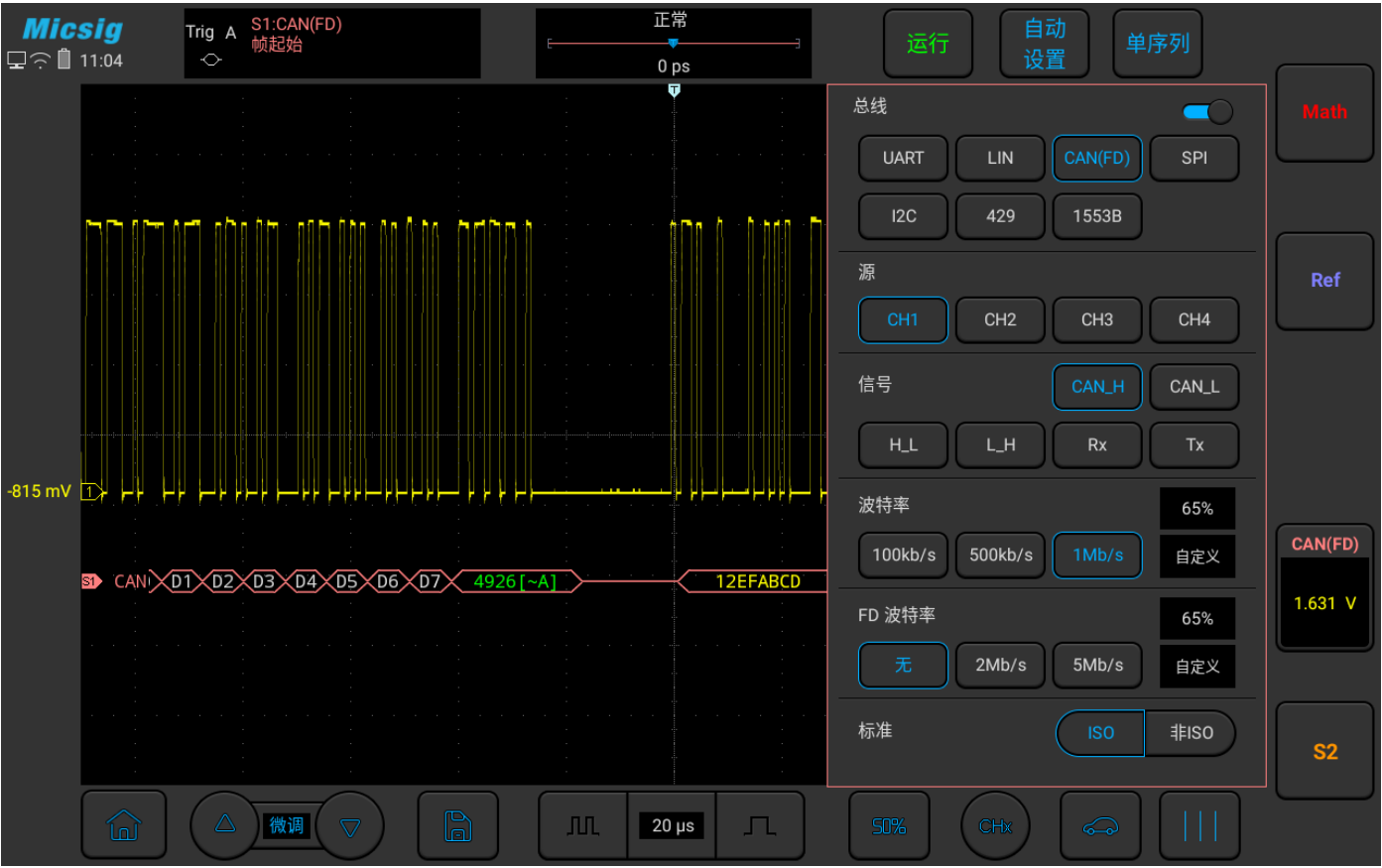
图12-14 CAN 总线配置菜单
