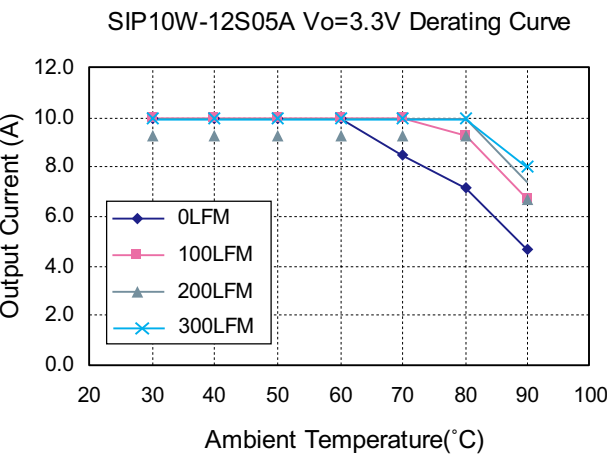
Figure3. Typical Power De-rating for 12Vin
