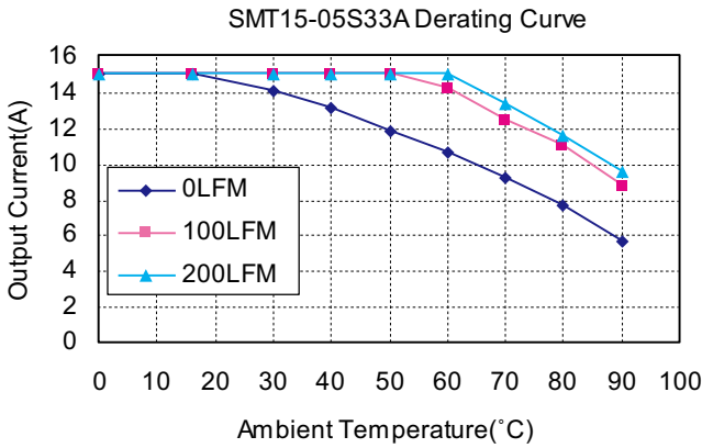
Figure3. Typical Power De-rating for 5Vin
