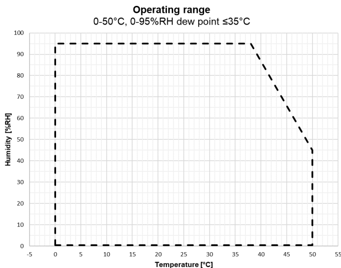
Figure 3 Operating range for specified in Table 1 accuracy.
