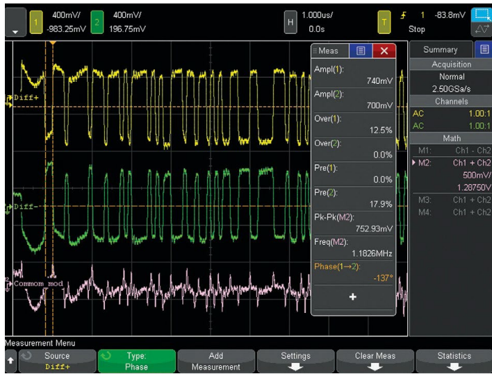
Figure 24. Dual channel WaveGen output of differential arbitrary signals. Common mode is shown as a math.
