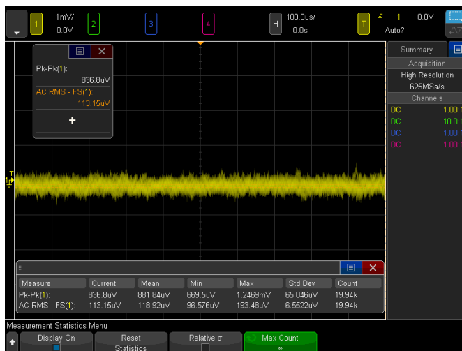
Figure 40. Getting 113 \mu Vrms noise floor at 1 mV/div with the high-resolution mode.
