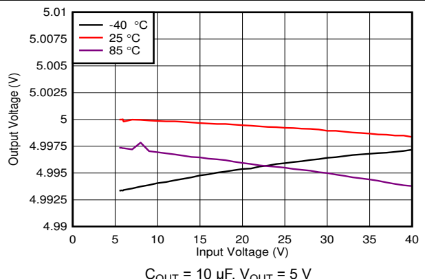
C_{OUT} = 10\ \mu\text{F} , V_{OUT} = 5\text{ V} 图 6-6. Line Regulation at 50 mA
