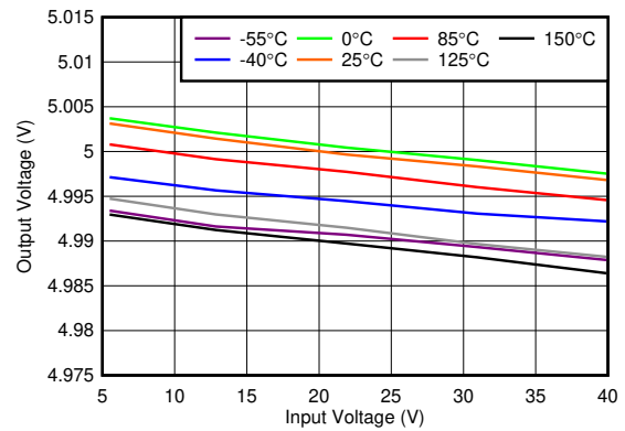
V_{OUT} = 5\text{ V} , I_{OUT} = 150\text{ mA} 图 6-2. Line Regulation vs V_{IN}
