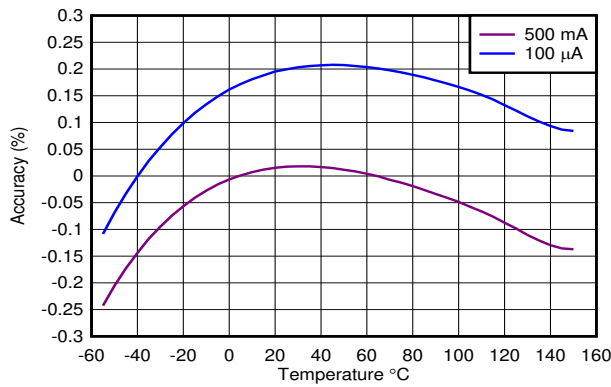
图 6-1. Accuracy vs Temperature
