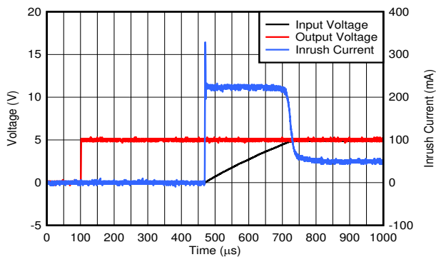
V_{IN} = 13.5\ \text{V} , C_{OUT} = 10\ \mu\text{F} 图 6-29. Startup Plot With EN
