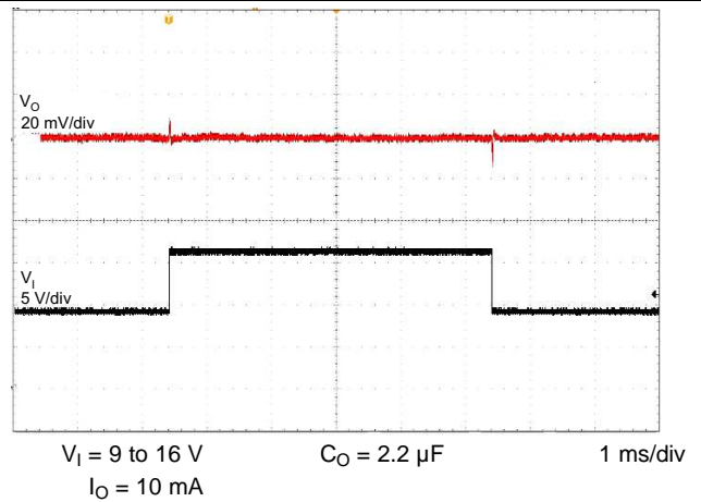
Figure 20. Line Transient ( V_O = 3.3 V)
