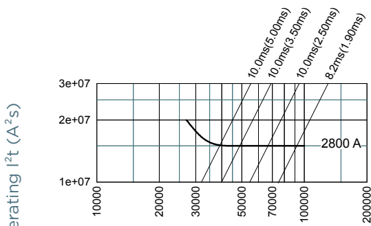
50Hz RMS symmetrical prospective current (Ip)(A)
