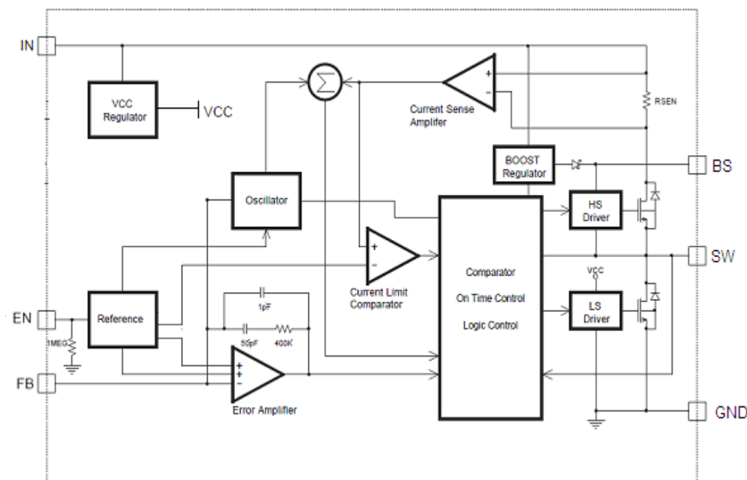
Figure 2. CP3471 Block Diagram
