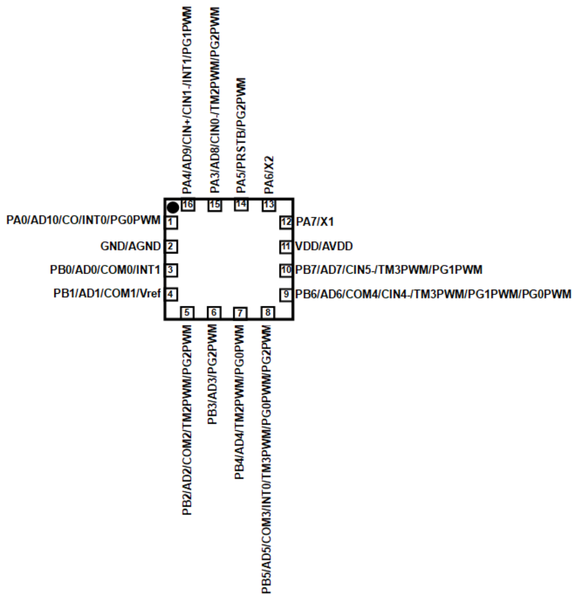
PFS123-1J16A (QFN3*3-16P-0.5pitch)
