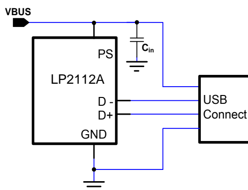
Figure 1. Typical Application Circuit of LP2112A with SOT23 6 Package Type.
