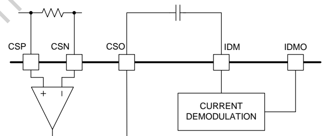
Fig2. Current Demodulation
