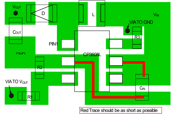
Figure 3. CP3608L Suggested Layout
