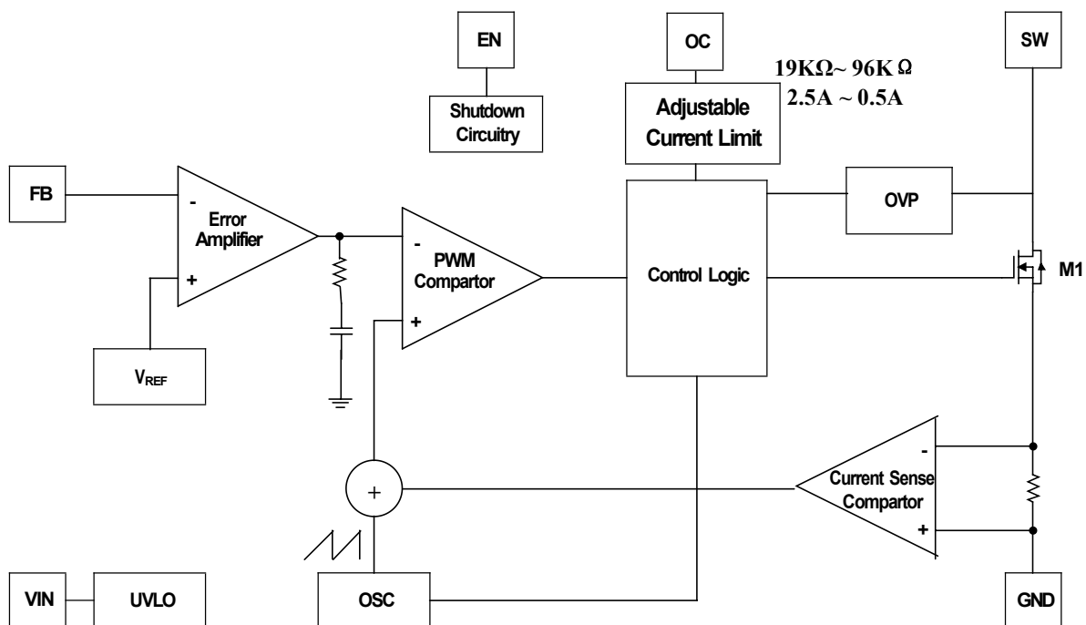
Figure 2. CP3608L Block Diagram
