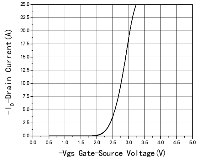
Fig2 Transfer Characteristics
