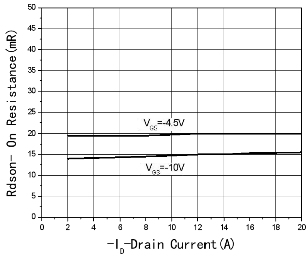
Fig3 Rdson-Drain current
