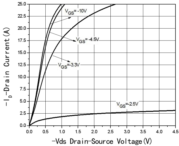
Fig1 Output Characteristics
