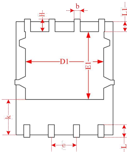
Bottom View
