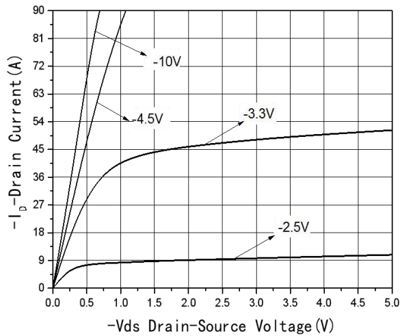
Fig1 Output Characteristics
