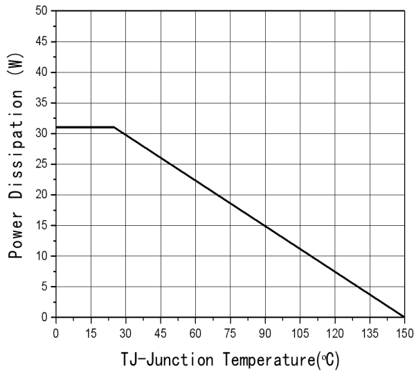
Fig7 Power De-rating
