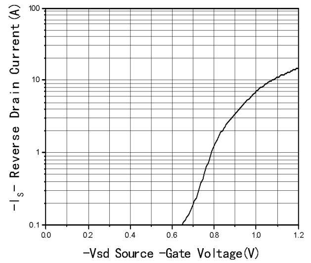
Fig8 Source-Drain Diode Forward
