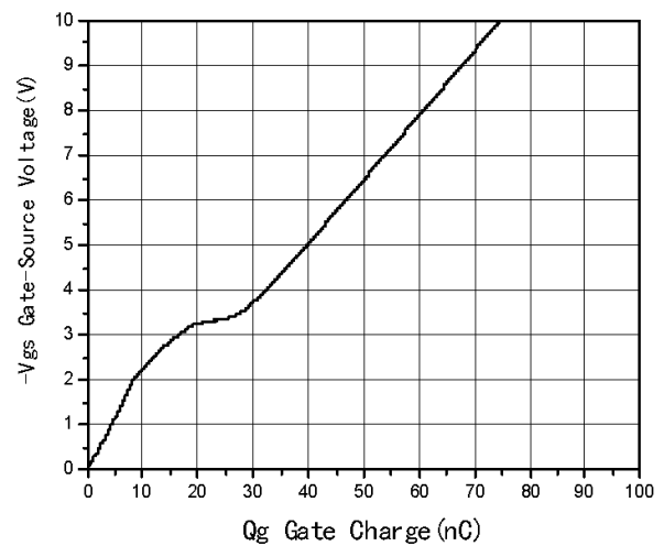
Fig6 Gate Charge
