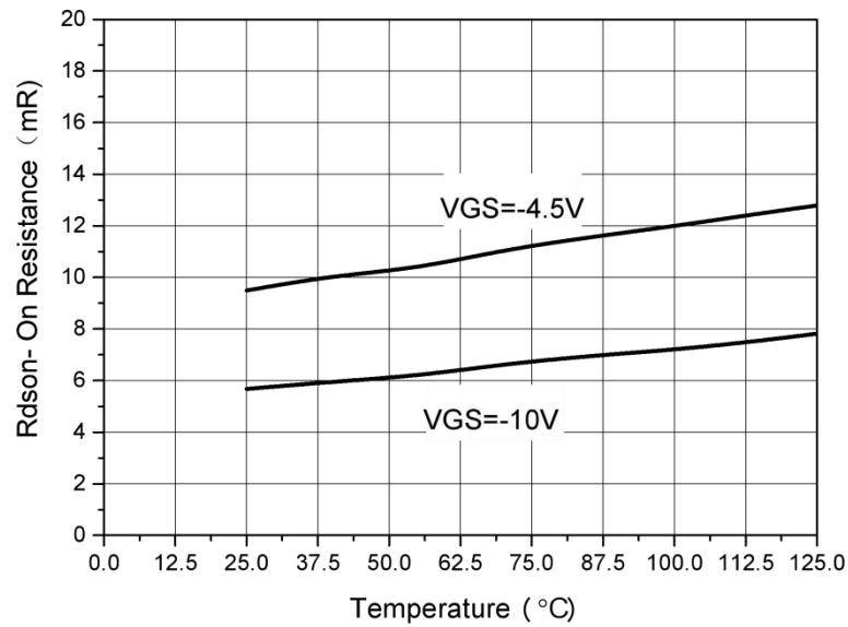
Fig9 Rdson vs Junction Temperature
