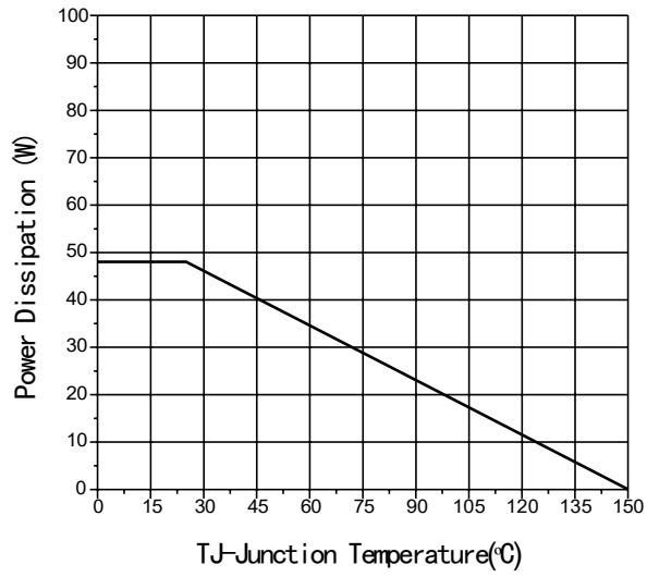
Fig7 Power De-rating
