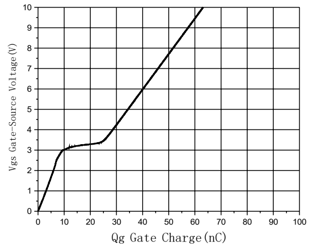
Fig6 Gate Charge
