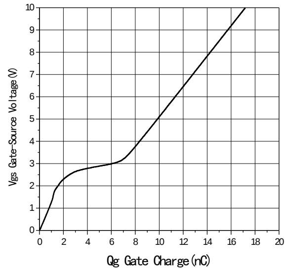
Fig6 Gate Charge
