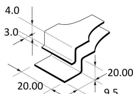
Dimensions mm
