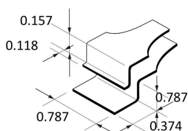
Dimensions inch
