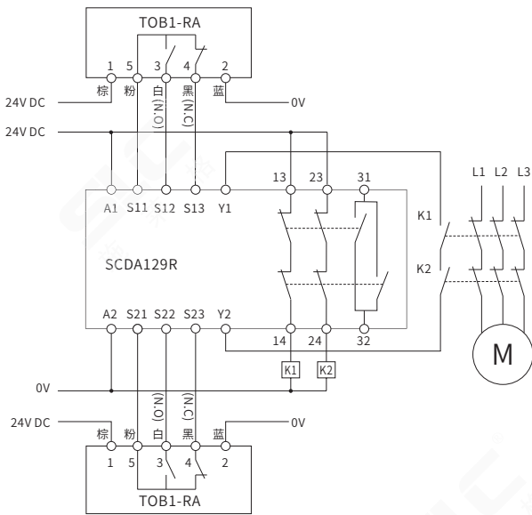
TOB1-RA与SCDA129R接线图
