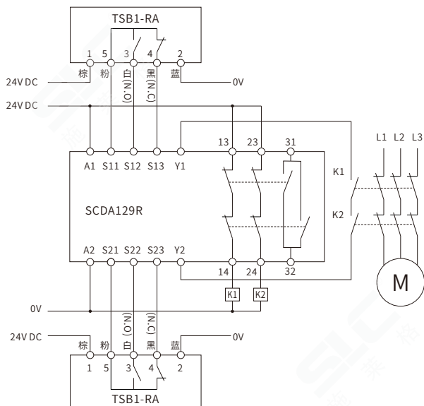
TSB1-RA与SCDA129R接线图
