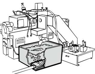
电镀液搅拌装置 / Liquid Mixer Bubbling
