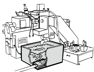
电镀液搅拌装置 / Liquid Mixer Bubbling
