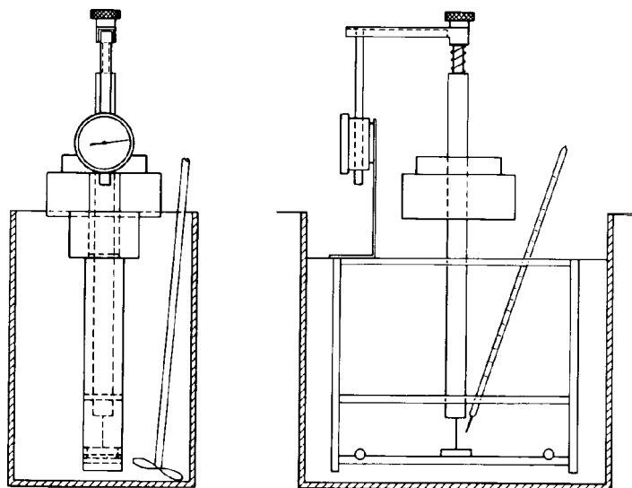
FIG. 1 Apparatus for Softening Temperature Determination
