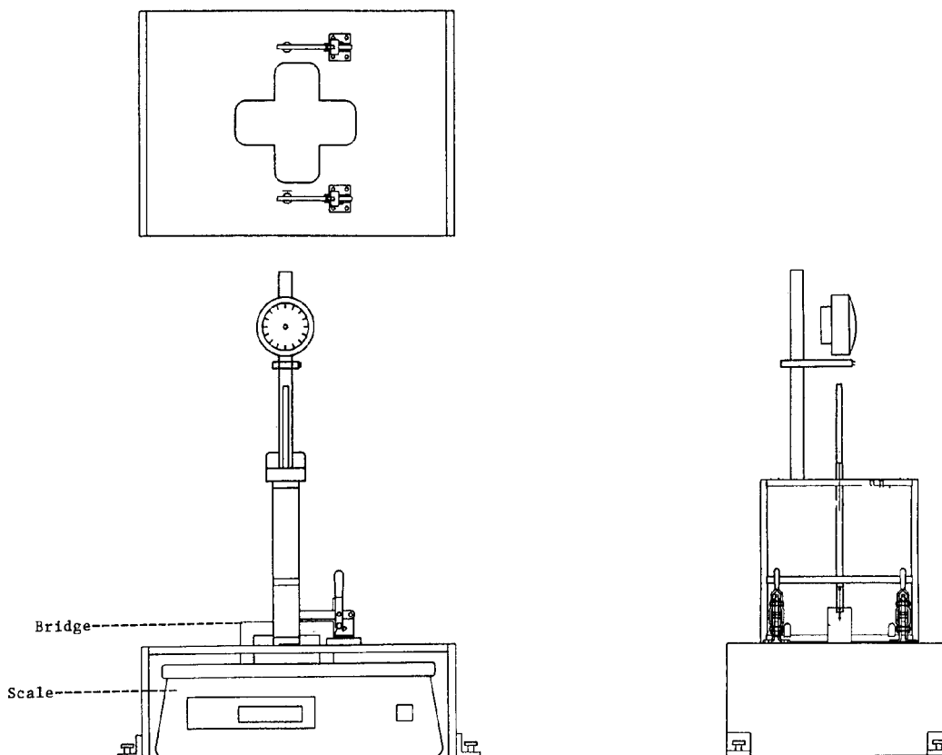
FIG. X1.1 Calibration Apparatus Using a Laboratory Scale
