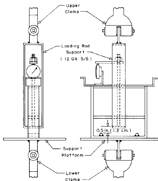
FIG. X2.1 Calibration Apparatus Using a Tensile Machine
