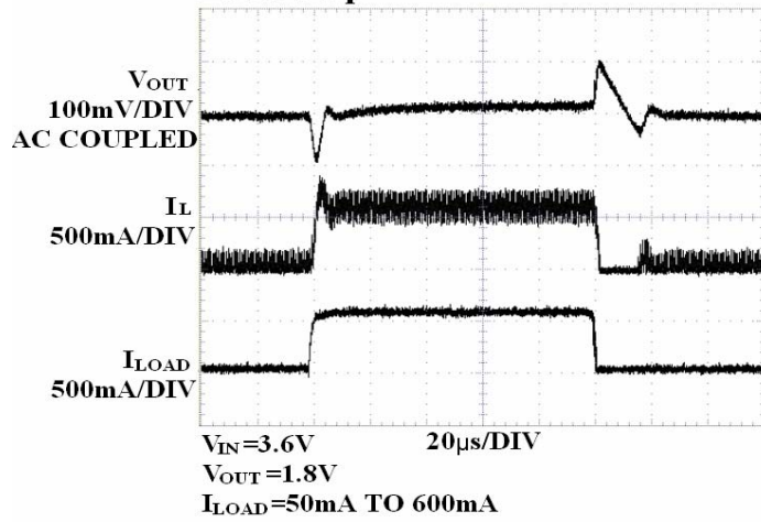
Load Step
