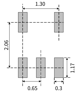
SC-70-5
