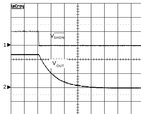
Entering Shutdown
