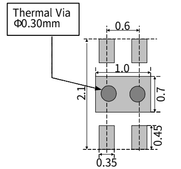
VTDFN1.2x1.6-4
