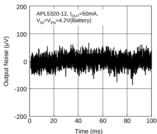
Output Noise
