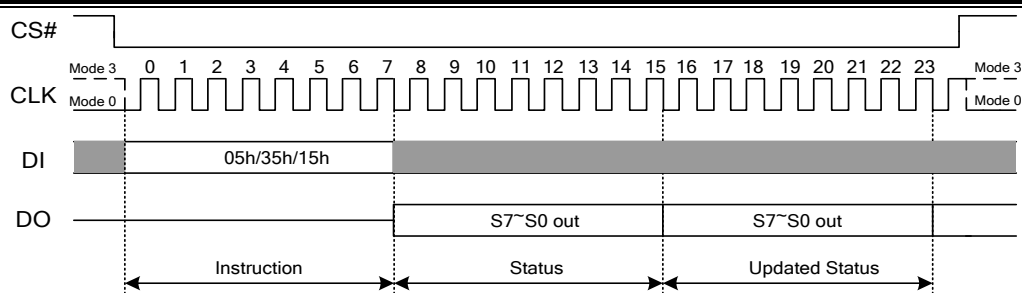
Figure 7.1 Read Status Register Instruction
