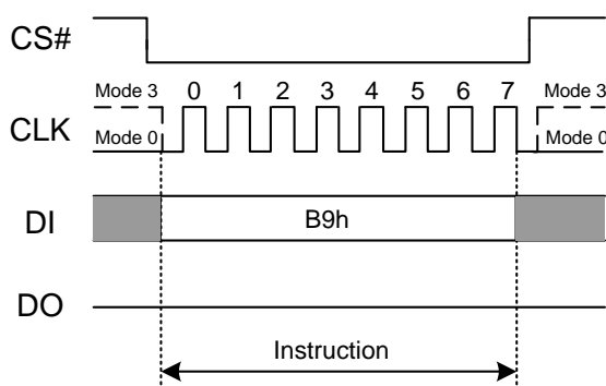
Figure 7.23 Deep Power-down Instruction
