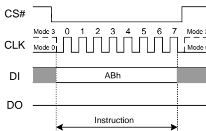
Figure 7.24 Release Power-down Instruction
