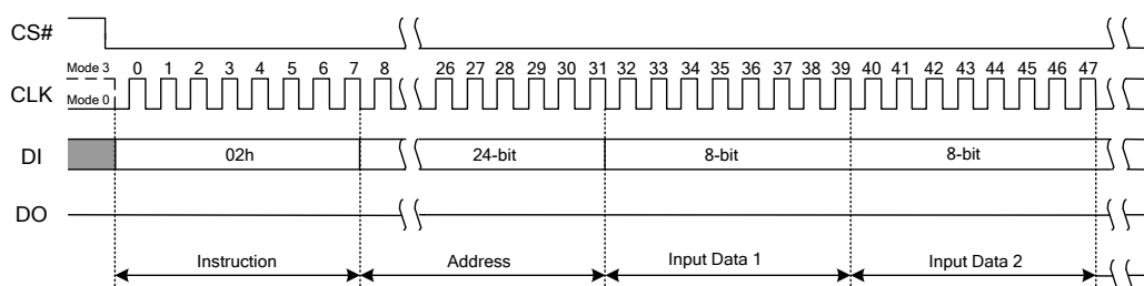
Figure 7.6 Page Program Instruction
