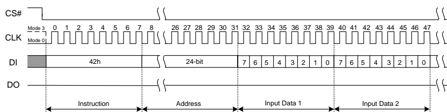
Figure 7.32 Program Security Registers Instruction
