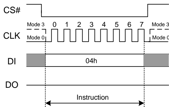
Figure 7.4 Write Disable Instruction
