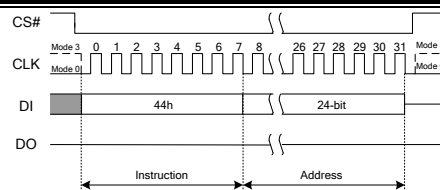
Figure 7.31 Erase Security Registers Instruction
