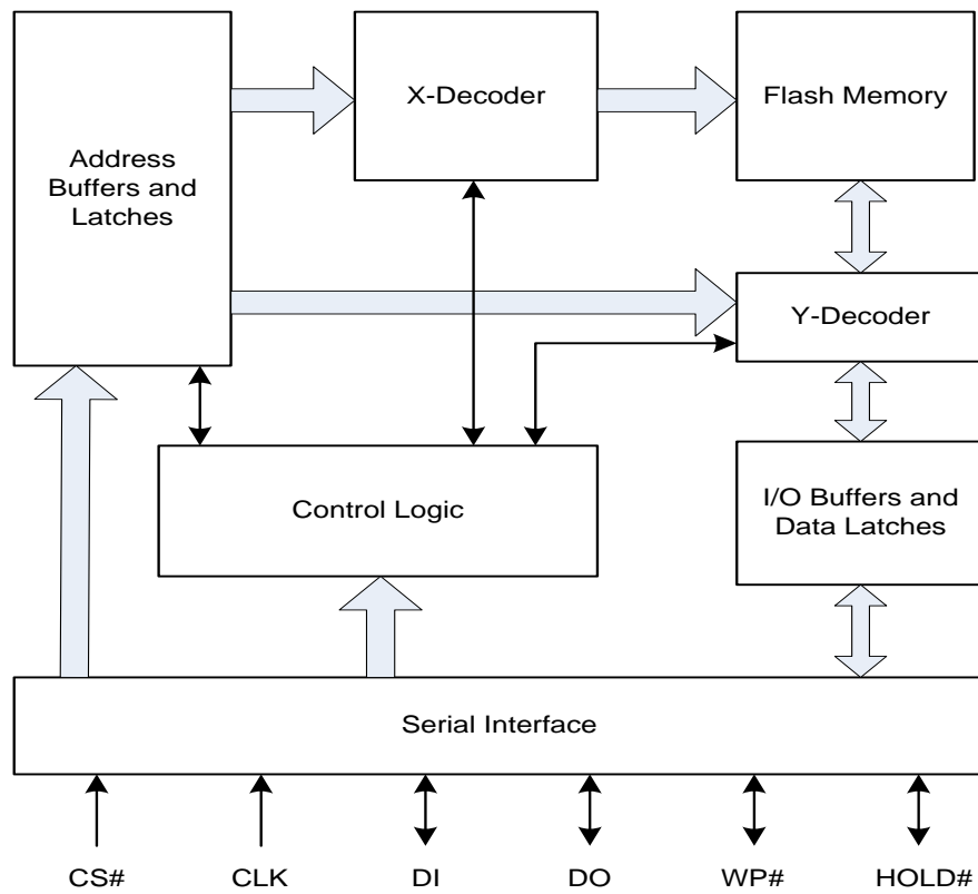
Figure 2.1 Block Diagram
