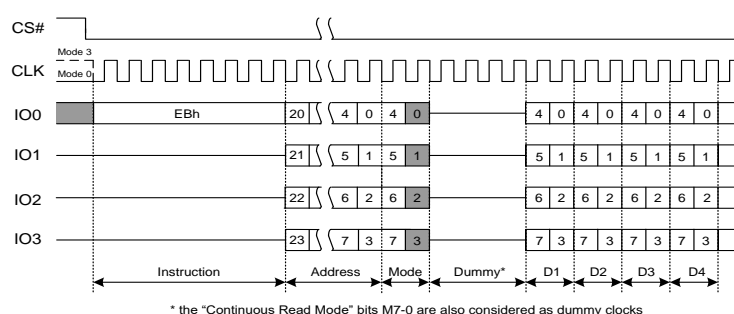
Figure 7.19 Fast Read Quad I/O Instruction(Initial command or previous M5-4 ≠10)
