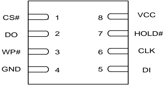
Figure 3.2 Table 3.1DFN8
