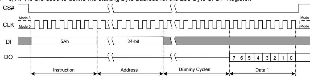
Figure 7.28 Read SFDP Register Instruction
