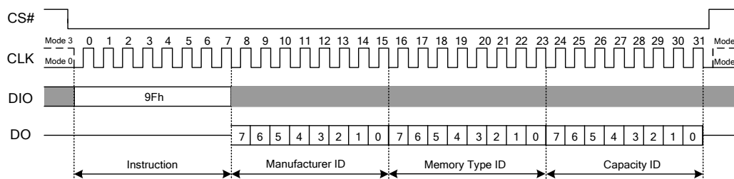
Figure 7.27 Read JEDEC ID
