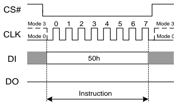
Figure 7.3 Write Enable for Volatile Status Register Instruction
