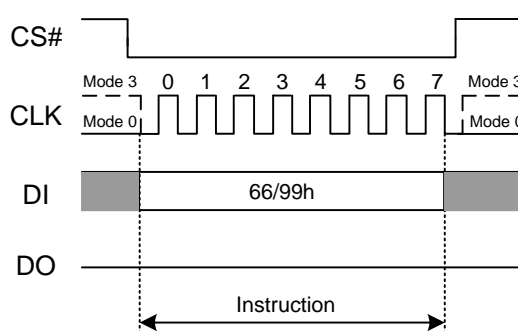
Figure 7.22 Software Reset Instruction
