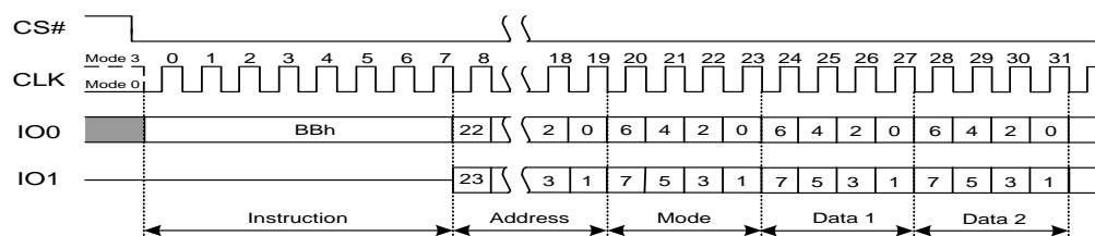
Figure 7.17 Fast Read Dual I/O Instruction (Initial command or previous M5-4≠10)
