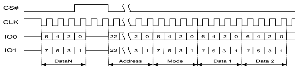
Figure 7.18 Fast Read Dual I/O Instruction (Initial command or previous M5-4=10)
