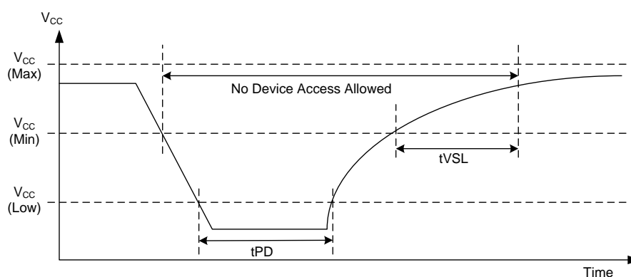
Figure 8.2 Power-Down and Voltage Drop
