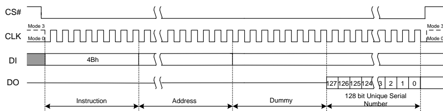
Figure 7.34 Read unique ID Number Instruction
