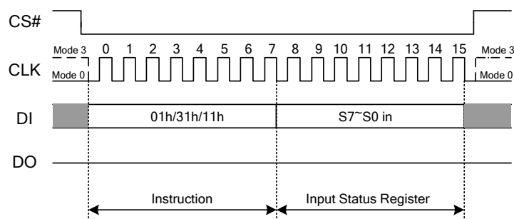
Figure 7.5 Write Status Register Instruction(SPI Mode)
