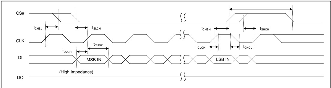
Figure 8.5 Input Timing
