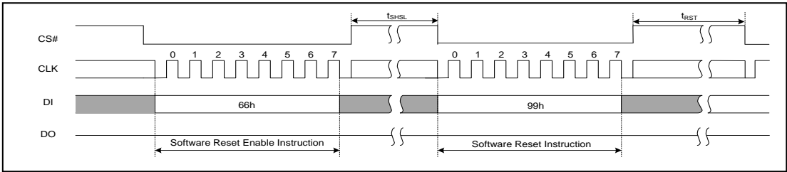
Figure 8.4 Serial Output Timing
