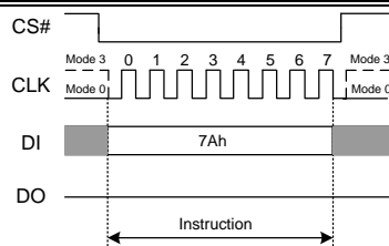
Figure 7.12 Erase/Program Resume Instruction
