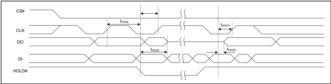
Figure 8.6 Hold Timing
