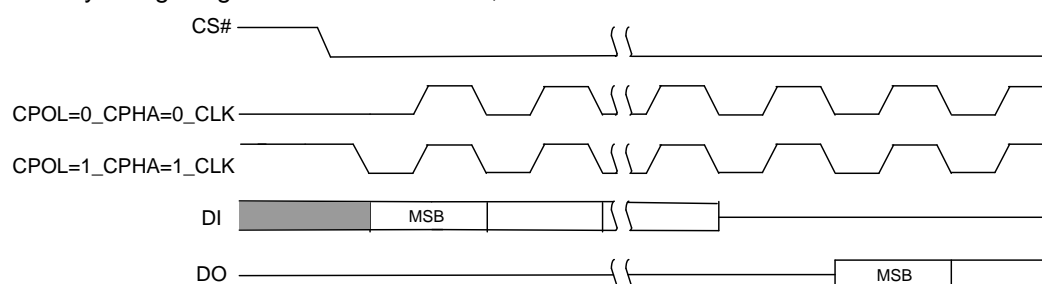
Figure 6.1 SPI Modes
