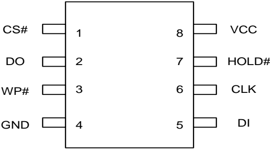
Figure 3.1 SOP8
