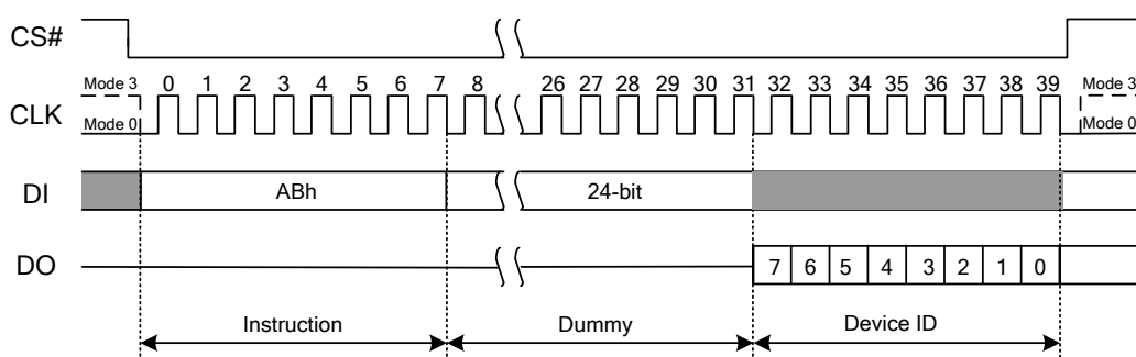
Figure 7.25 Release Power-down / Device ID
