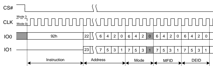
Figure 7.29 Read Manufacturer/Device ID Dual I/O Instruction
