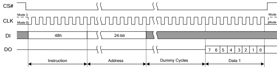
Figure 7.33 Read Security Registers Instruction
