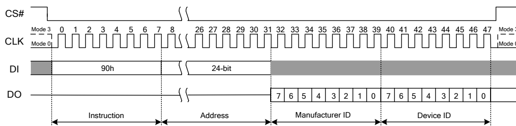
Figure 7.26 Read Manufacturer/Device ID
