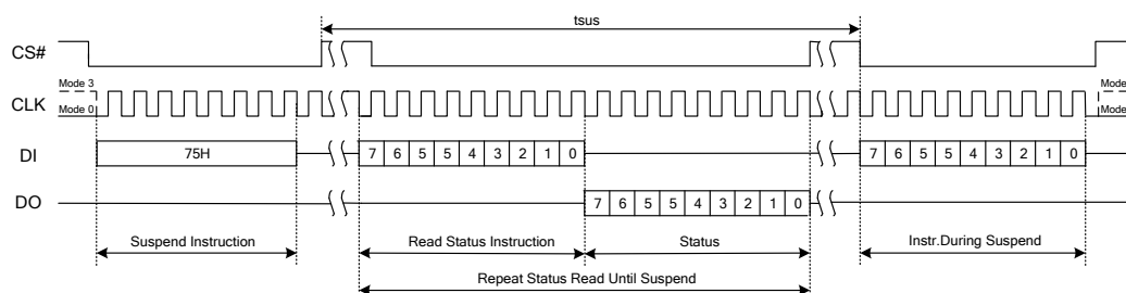
Figure 7.11 Erase / Program Suspend Instruction
