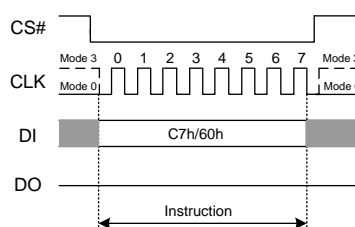
Figure 7.10 Chip Erase Instruction
