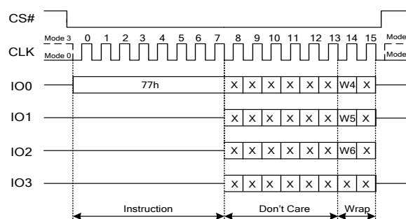
Figure 7.21 Set Burst with Wrap Instruction
