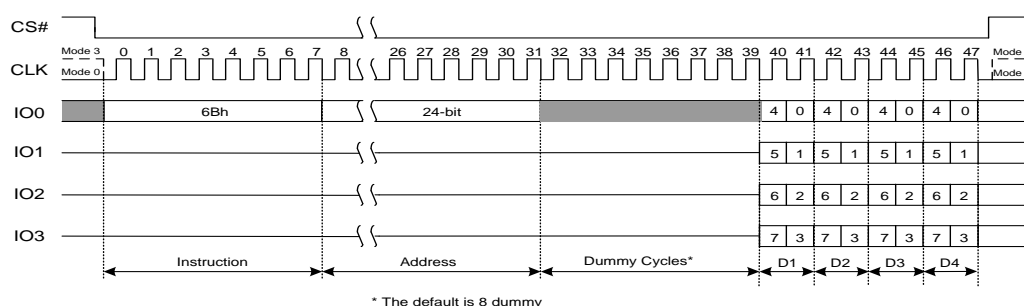
Figure 7.16 Fast Read Quad Output Instruction
