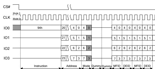
Figure 7.30 Read Manufacturer/Device ID Quad I/O Instruction
