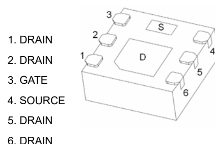
DFNWB2×2-6L-J
