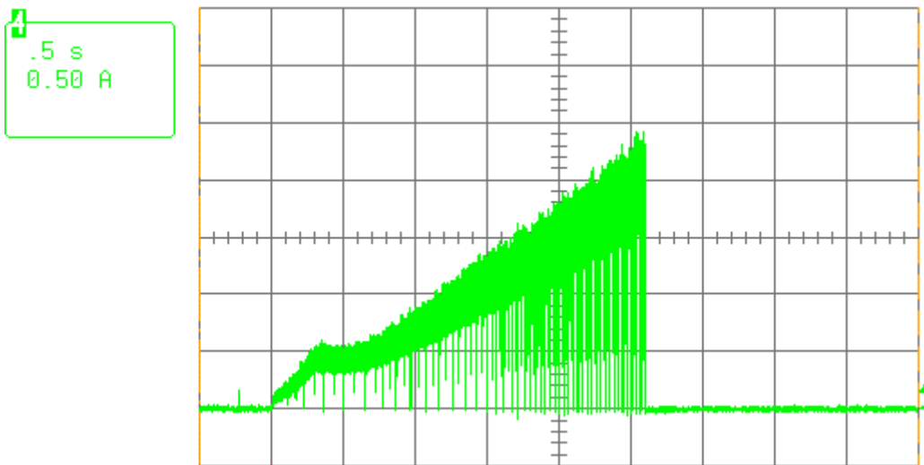
Locked rotor current at 24 V
